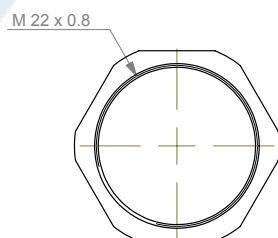
REP 3: Ecrou M 22 (Nut M 22)
